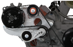
A/C Brackets (508) ICT# 551474
