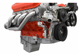
551169/551169-LS01 (Shown) LS Front Engine Plate Support Brace Kit $74.99-$99.99
