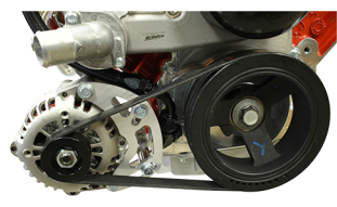
551177LS0 LS Alternator bracket for Electric Water Pumps $299.99
